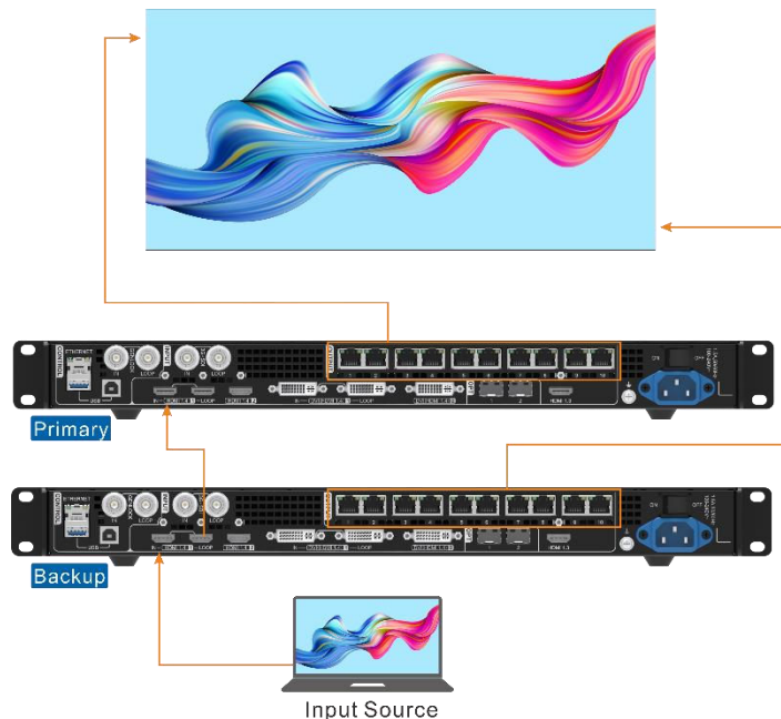
Figure 5-25 Device backup connection
