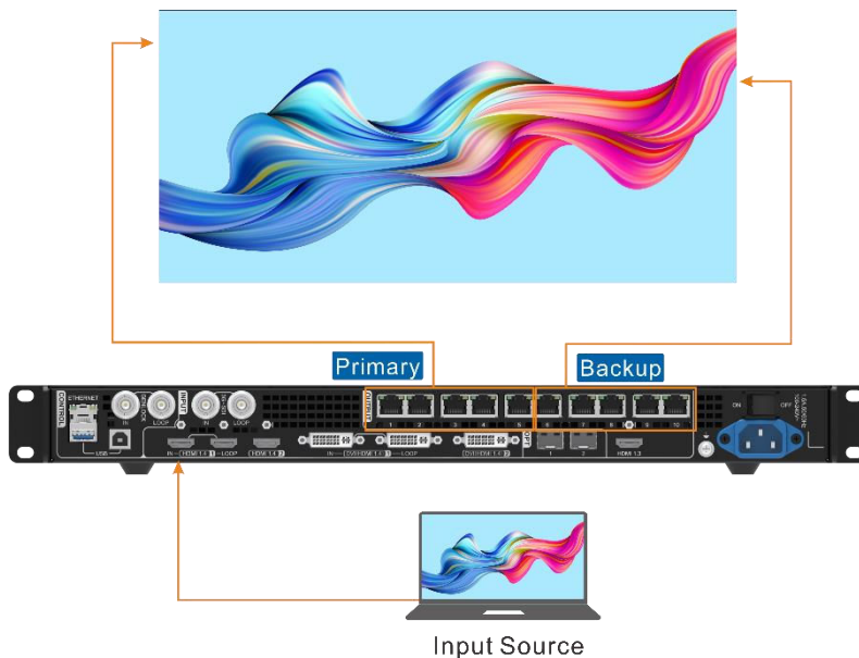
Figure 5-27 Ethernet port backup connection
