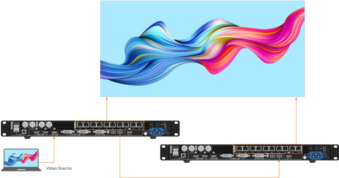
Figure 5-43 Backup
